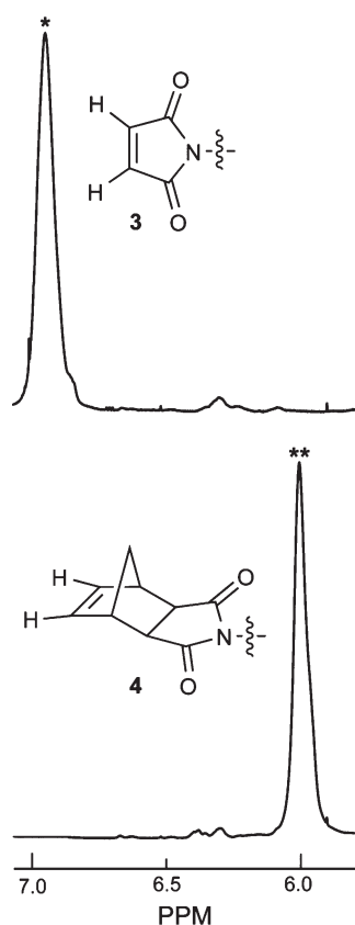
Figure 1. ^1\text{H} NMR spectra of maleimide-containing polymer 3 and norbornene-containing polymer 4 . A region diagnostic of polymer modification is shown before ( 3 ) and after ( 4 ) the Diels–Alder reaction with cyclopentadiene. The spectra show that the olefinic protons of the maleimide groups (*) disappear and olefinic protons of norbornene moieties (**) appear, indicating that the conversion of 3 to 4 proceeds in high yield.
